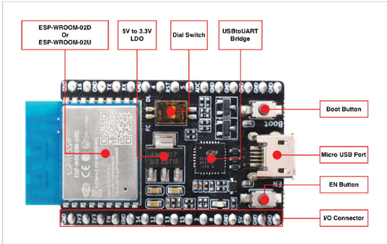
Fig. 2: ESP8266-DevKitC with ESP-WROOM-02D module soldered
